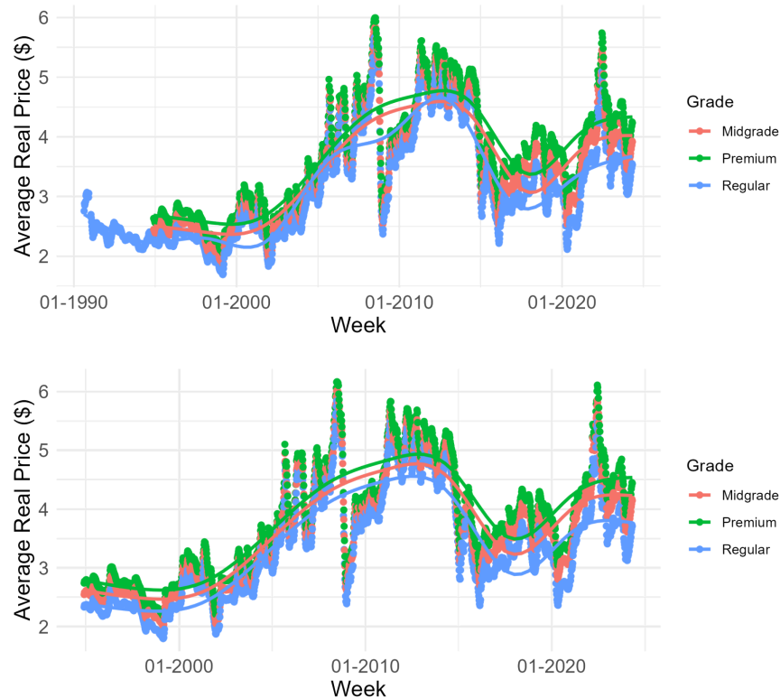
Figure 2: Avg. Weekly Real Prices for Conventional (Top) and Reformulated (Bottom) Gasoline
