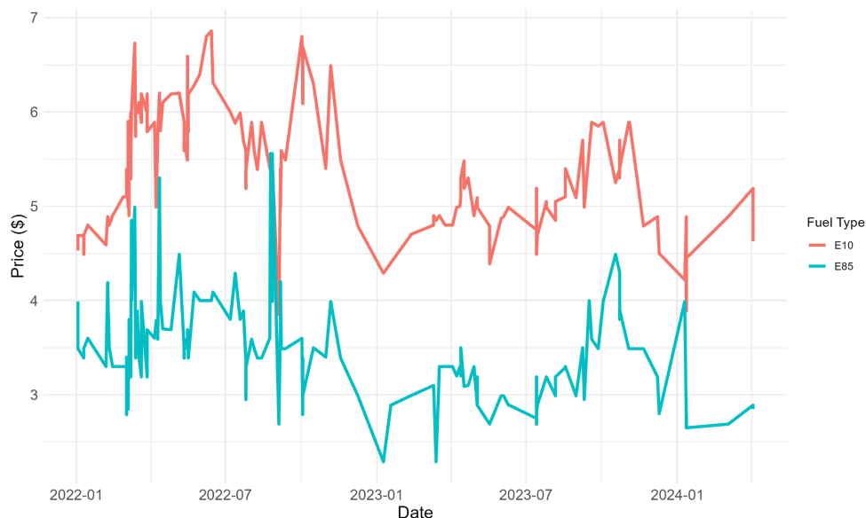
Figure 7: Prices of E10 and E85 in California
