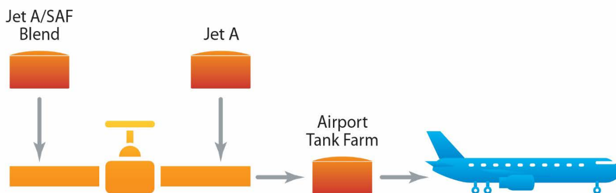
Figure 11. Alternative method of blending Jet A and SAF at a terminal
