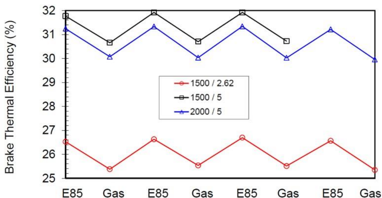
FIGURE 4: EFFECT OF E85 ON ENGINE EFFICIENCY
