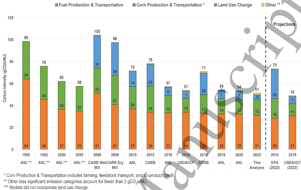
Figure 1. Timeline of estimated corn ethanol life cycle greenhouse gas emissions for 1990 through 2020 with projections out to 2022.
