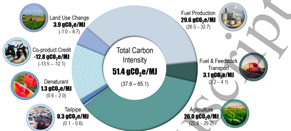
Figure 5. Greenhouse gas emission categories and total carbon intensity of corn ethanol.
